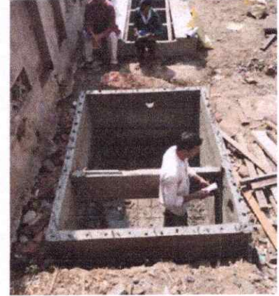
Figure 3 Septic Tank
